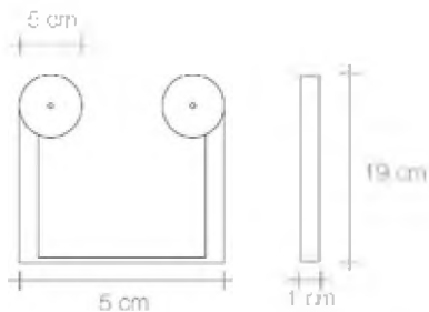
Z0120800 Staffa muro / Wall clamp
